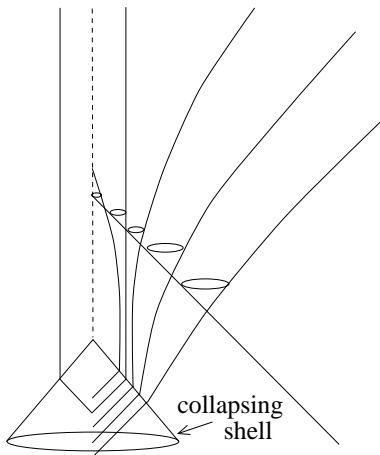
Figure 1.2: Picture of a black hole that forms from a collapsing shell of matter.
