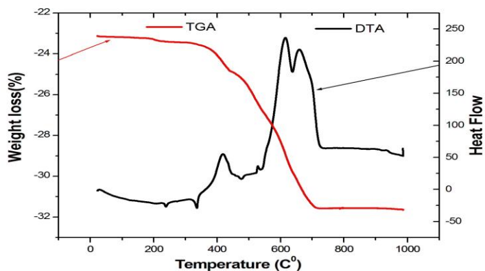
Figure 1. TGA and DTA curves of dmphen-CdI 2 complex.
