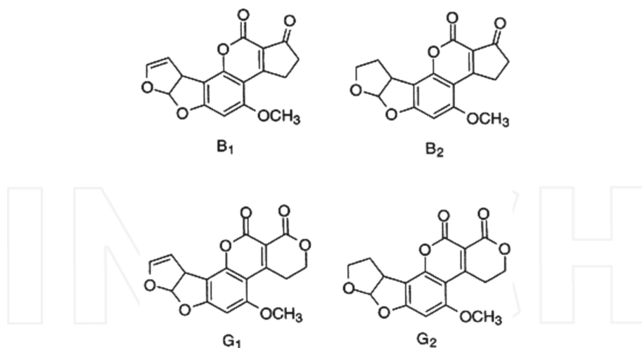
Figure 4. Chemical structures of the four major naturally produced aflatoxins: aflatoxin B 1 , aflatoxin B 2 , aflatoxin G 1 , and aflatoxin G 2 .
