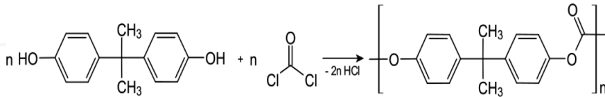
Figure 2. Synthesis of the polymer polycarbonate from bisphenol A and phosgene.
