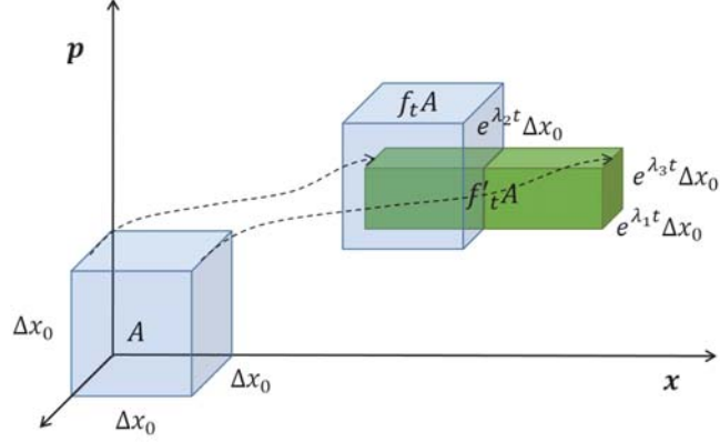
Figure 1: Schematic illustration of the phase space evolution in both the regular and the chaotic case. An infinitesimal element A of volume (\Delta x_0)^n , where n is the dimension of the phase space, evolves in f_t A under a regular flow or in f'_t A under a chaotic flow. The volume of the overlap between the two evolved elements has the linear size of \Delta x_0 along all directions of divergence and e^{\lambda_i t} \Delta x_0 ( \lambda_i < 0 ) for every direction i of contraction.
