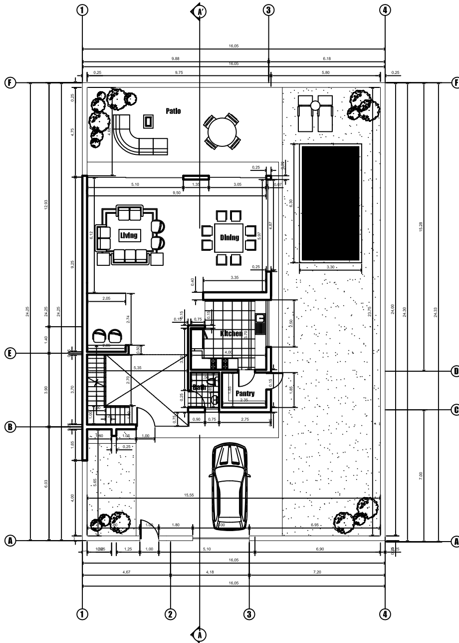
GROUND FLOOR PLAN Scale 1:200
