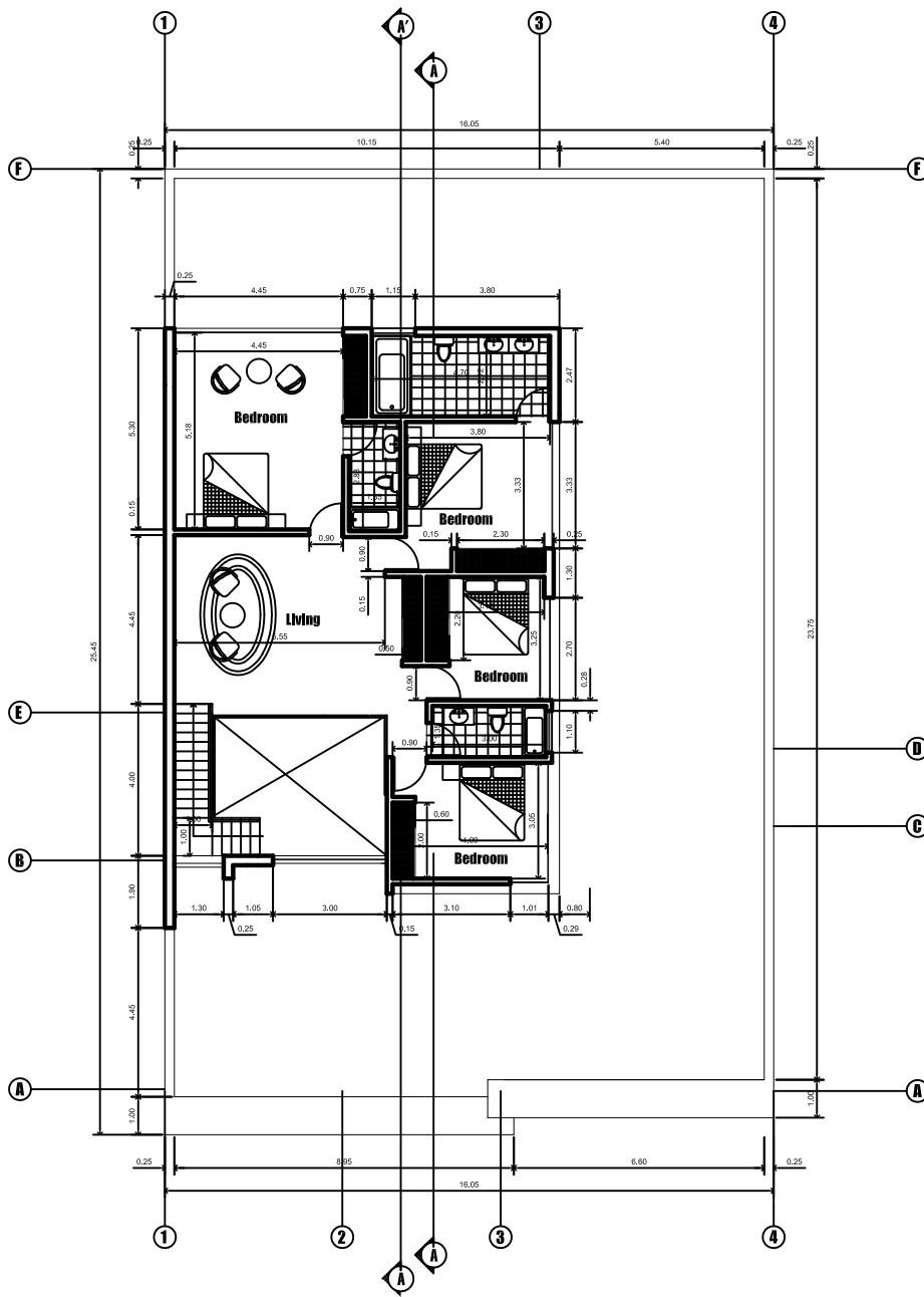
FIRST FLOOR PLAN Scale 1:200
