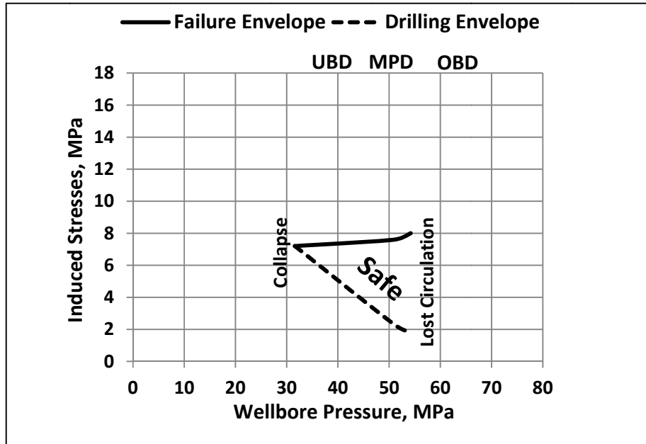
Fig. 4 Vertical well in very weak formation (R1)
