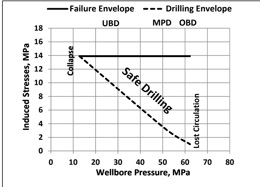
Fig. 8 Horizontal well ( //\sigma_H ) in medium strong formation (R3)
