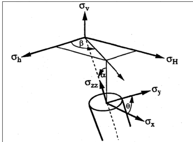
Fig. 2 Stresses transformation for a directional well
