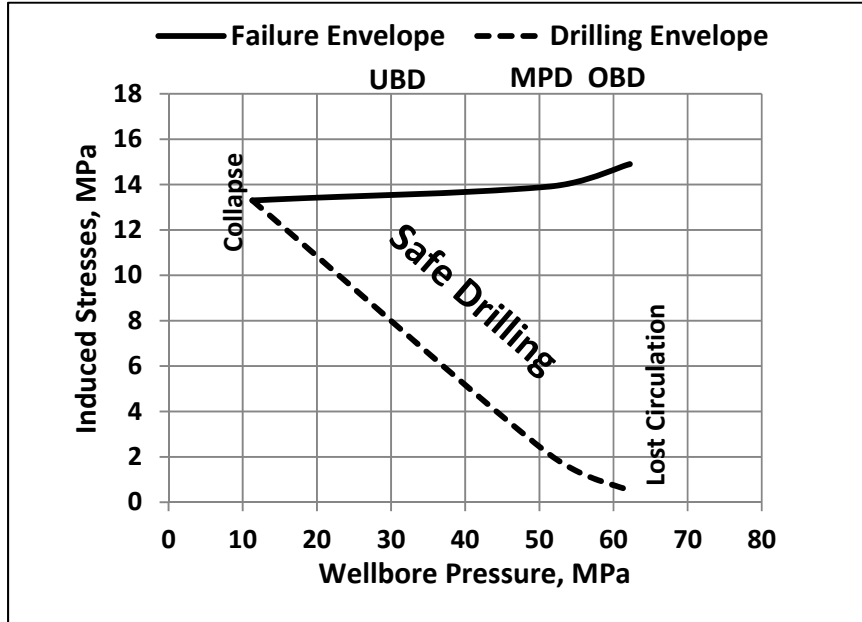
Fig. 6 Vertical well in medium strong formation (R3)
