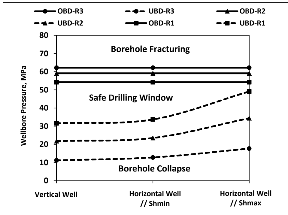
Fig. 10 Safe drilling in three different horizontal well orientations and formations strengths
