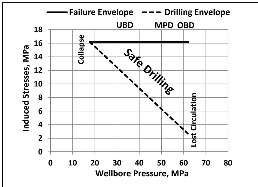
Fig. 9 Horizontal well ( //\sigma_h ) in medium strong formation (R3)
