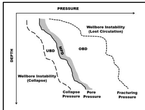
Fig. 1 Drilling windows for various types of drilling operations
