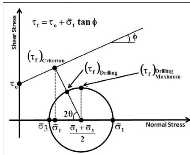
Fig. 3 Representation of drilling induced failure possibility
