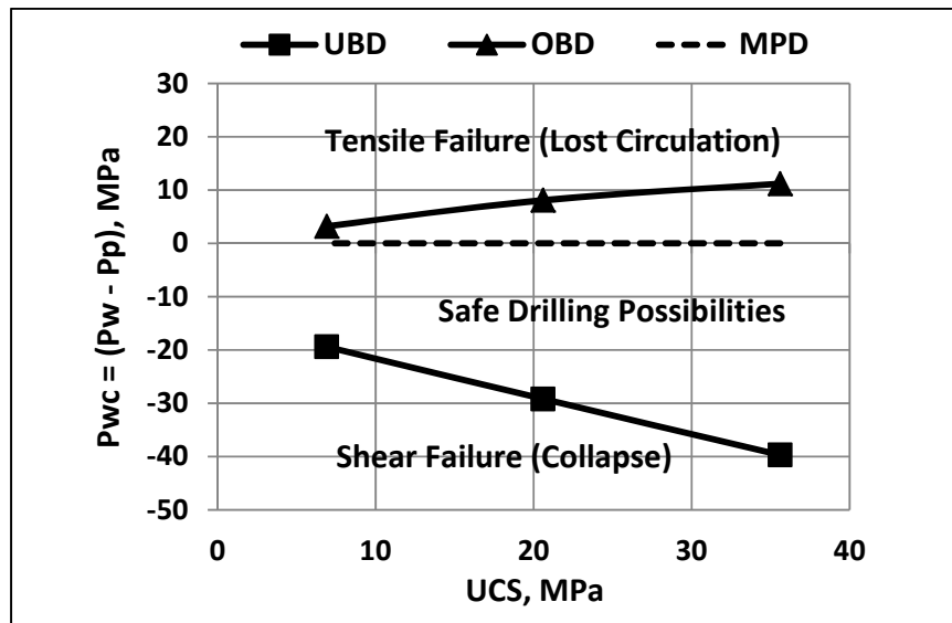
Fig. 7 Summary of the studied vertical drilling cases
