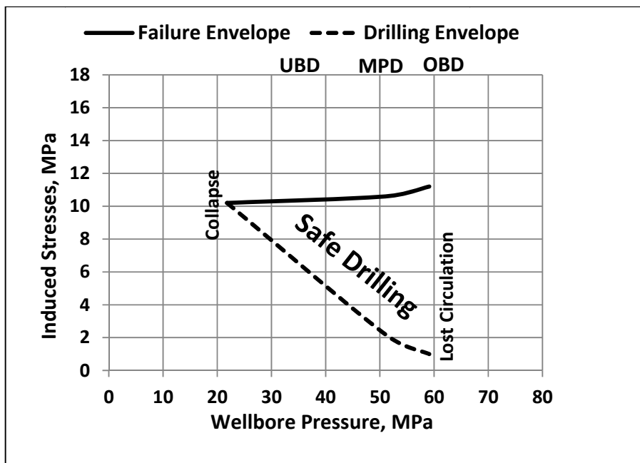
Fig. 5 Vertical well in weak formation (R2)
