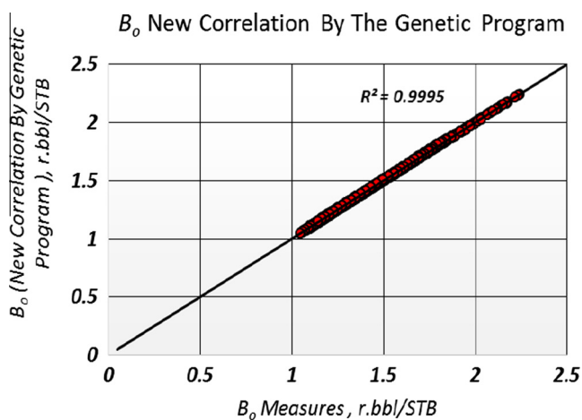
Figure 7 Crossplot of measured and new generated B_o correlation by genetic program for volatile oil samples.
