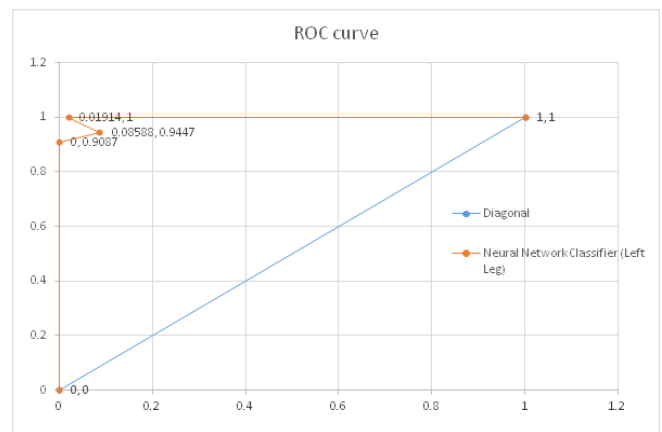
Figure 6 ROC curve of Neural Network classifier for Left Leg Data
