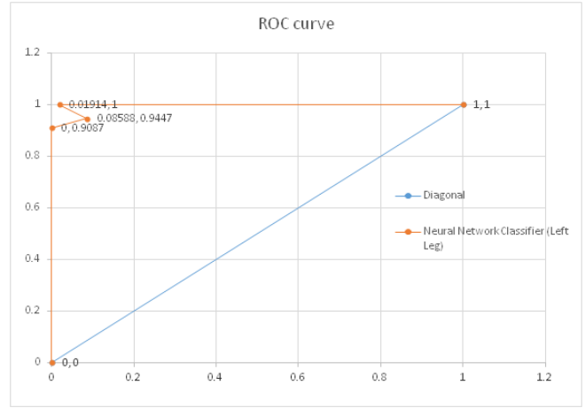
Figure 5 ROC curve of Neural Network classifier for Left Leg Data
