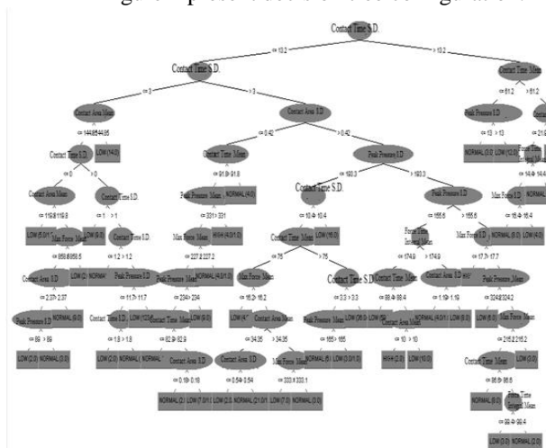
Figure 4 Decision Tree Example for Classify Data.
