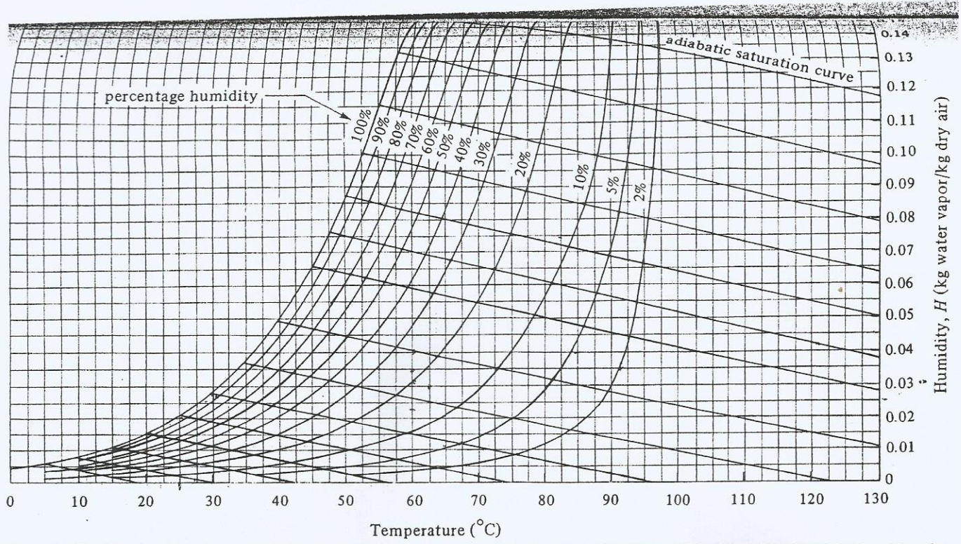
FIGURE 9.3-2. Humidity chart for mixtures of air and water vapor at a total pressure of 101.325 kPa (760 mm Hg). (From R. E. Treybal, Mass-Transfer Operations , 3rd ed. New York: McGraw-Hill Book Company, 1980. With permission.)
