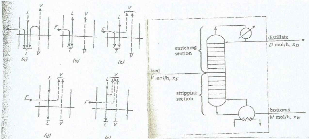
Figure 18-13 Flow through feed plate for various feed conditions: (a) feed cold liquid; (b) feed saturated liquid; (c) feed partially vaporized; (d) feed saturated vapor; (e) feed superheated vapor.
