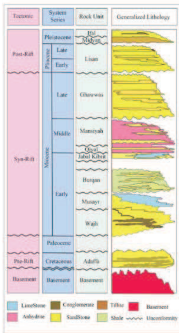
Figure (2) Generalized chronolithostratigraphic succession of the Midyan region (modified after Wyn Hughes and Johnson, 2005 and Laboun, 2011).
