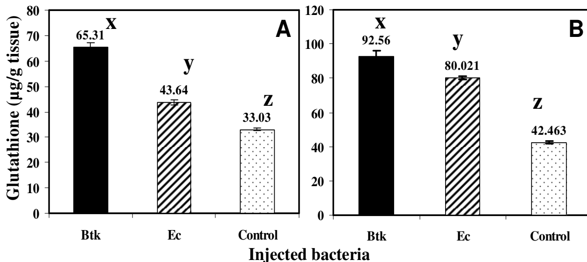
Figure 3. Titer of glutathione (GSH) ( \mu\text{g/g} mosquito tissue) in 5-days-old adult Ae. caspius mosquito at 12 h (A) and 24 h (B). Mosquitoes were challenged with B. thuringiensis kurstaki (Btk) or E. coli (Ec), or sham injected with APS (control). GSH titer was measured at 12 and 24 h post-treatment. Error bars represent standard error of means of 5 replicates ( N = 5 ). Within each experiment, different letters above bars (x, y and z) represent significant difference in the amounts of GSH ( \mu\text{g/g} mosquito tissue) comparing to control mosquitoes in each case ( P < 0.05 , ANOVA). Numbers on bars represent the amounts of GSH ( \mu\text{g/g} larval tissue).
