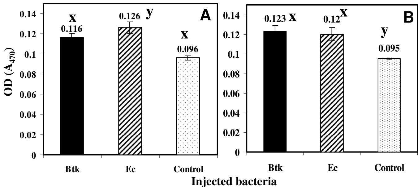
Figure 5. Titer of PO (absorbance (OD) at A 470 ) in adult autogenous Ae. caspius mosquitoes at 12h (A) and 24h (B) post-treatment. Five-days old mosquitoes were inoculated with B. thuringiensis kurstaki ( Btk ) or E. coli ( Ec ), or sham injected with APS (control). PO titer was measured at 12h and 24h post-treatment (OD measurements at A 470 ). Error bars represent standard errors of means of OD measurements at A 470 from five different independent assays (N = 5) in each case. Within each experiment, different letters above bars (x, y & z) represent significant difference comparing to control mosquitoes ( P < 0.05 , ANOVA) in OD measurements at A 470 in each case. Numbers on bars represent the means of OD measurements at A 470 .
