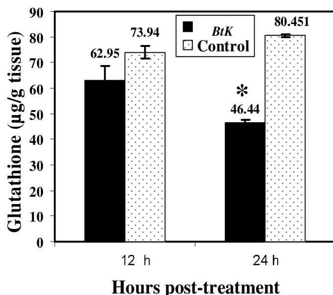
Figure 2. Glutathione (GSH) titer ( \mu\text{g/g} larval tissue) in the third larval instars of the autogenous Ae. caspius mosquito. Larvae were treated with \text{LC}_{50} of Btk spore-crystal powder or left without treatment (control). GSH titer was measured at 12 and 24h post-treatment. Error bars represent standard error of means of 5 replicates (N = 5). Asterisk (*) represents significant lower GSH titer comparing to control larvae ( P < 0.05 , two-sample t-test). Numbers on bars represent the amounts of GSH ( \mu\text{g/g} larval tissue).
