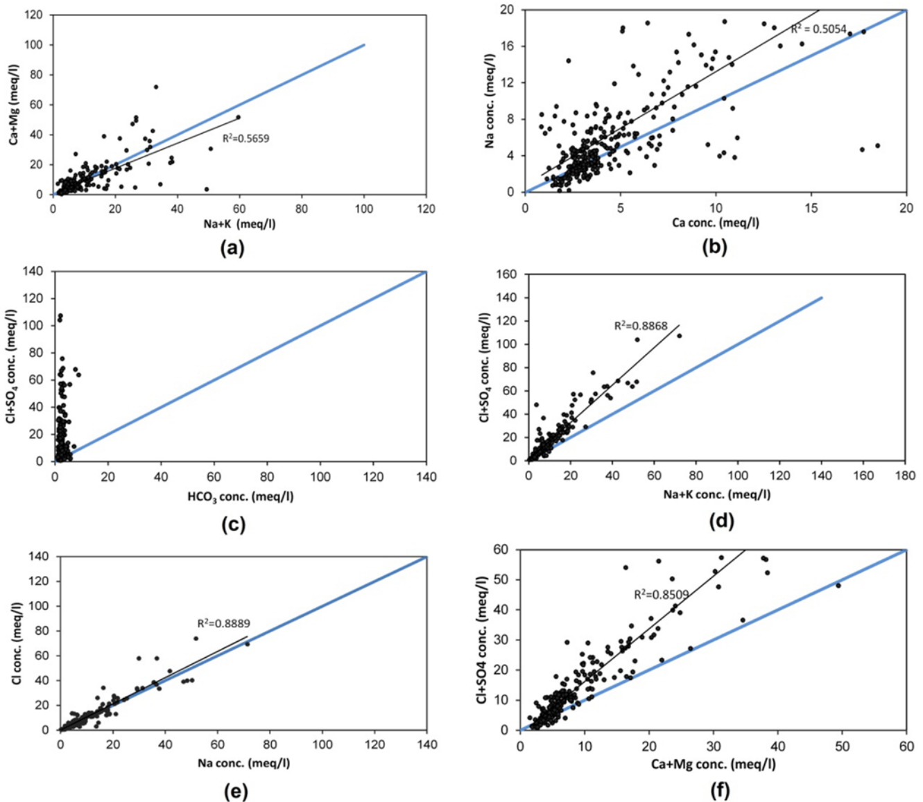
Fig. 3. Major ion chemistry of the Saq aquifer: (a) Alkalies relationship with Ca and Mg, (b) Ca versus Na relationship, (c) Relative abundance of weak ( \text{HCO}_3^- ) and strong ( \text{Cl}^- + \text{SO}_4^{--} ) acids, (d) Bonding affinity between Alkalies and \text{Cl}^- + \text{SO}_4^{--} , (e) Bonding relationship of Na-Cl, (f) Relationship of Ca + Mg with \text{Cl}^- + \text{SO}_4^{--} .
