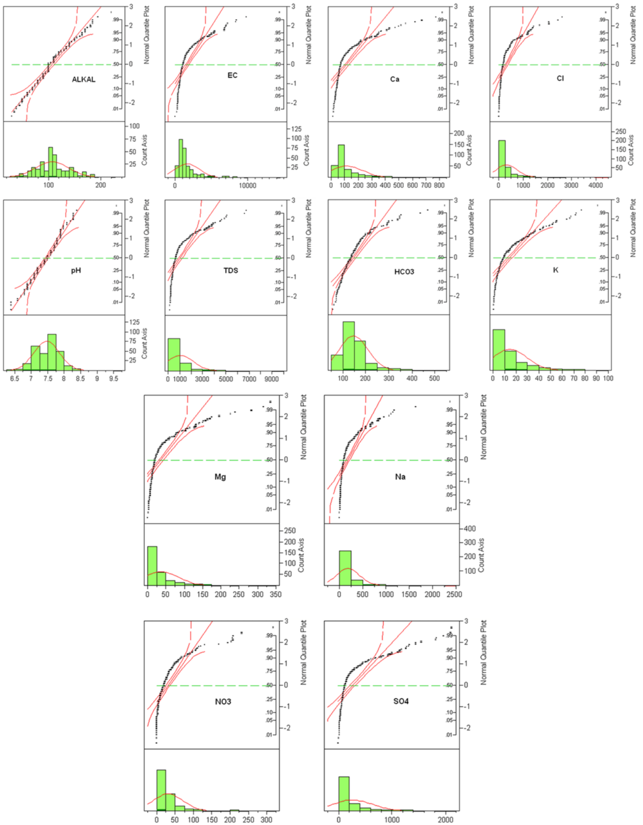
Fig. 4. Normal quantile plots (the normal quantiles are plotted on the y-axis; the observed values are plotted on the x-axis EC in [μS/cm]; chemical elements are in mg/L) and Histograms for the data set (a normal distribution curve for all the values is superimposed for comparison; EC in [μS/cm]; chemical elements are in mg/L).
