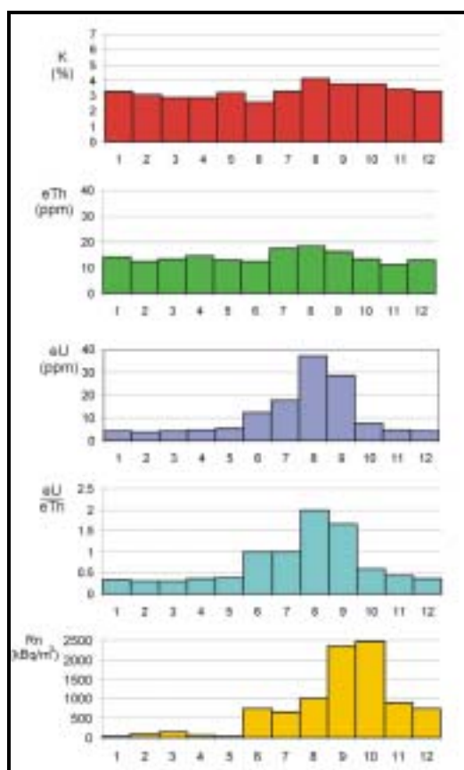
FIG. 9.5. K, U, Th concentrations and 222 Rn activity concentration over U mineralization in the Urt mineral zone, Mongolia (Matolin, 1994).
