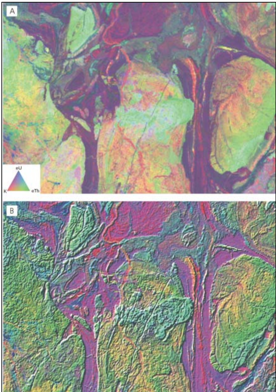
FIG. 7.15. (a) Ternary radioelement map H and S modulate relative radioelement abundance ( K = \text{red} , \text{Th} = \text{green} , U = \text{blue} ), I modulates total count channel; (b) IHS composite image, H and S modulate relative radioelement abundance, I modulates relief shaded total count channel (data courtesy of Geoscience Australia).
