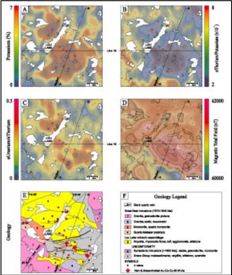
FIG. 9.6. Radiometric responses, magnetic response and the geology of the Lou Lake area, Northwest Territories, Canada. Polymetallic mineralization associated with potassium and magnetite-enriched hydrothermal system. Uranium enrichment occurs on the margins of the hydrothermal system (after Shives et al., 1997).
