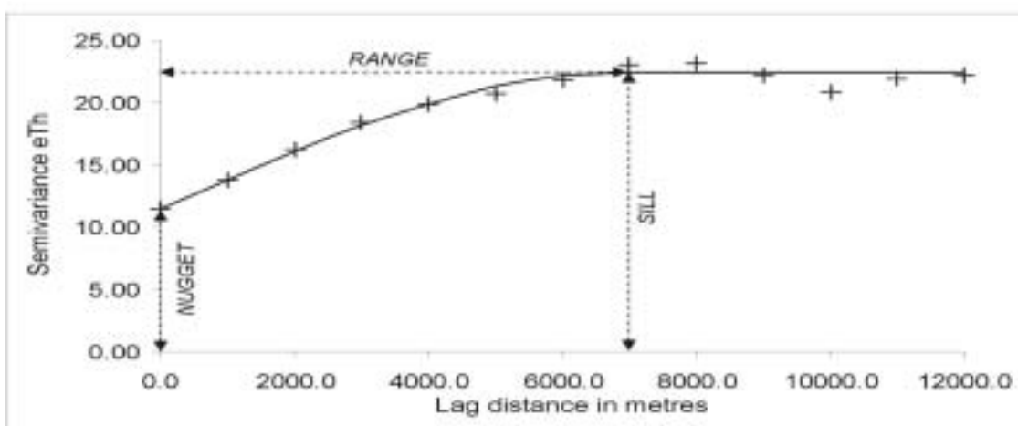
FIG. 7.5. Semivariogram plot of airborne eTh data fitted to a spherical model (nugget = 11.5, sill = 22.5 and range = 7000 metres).
