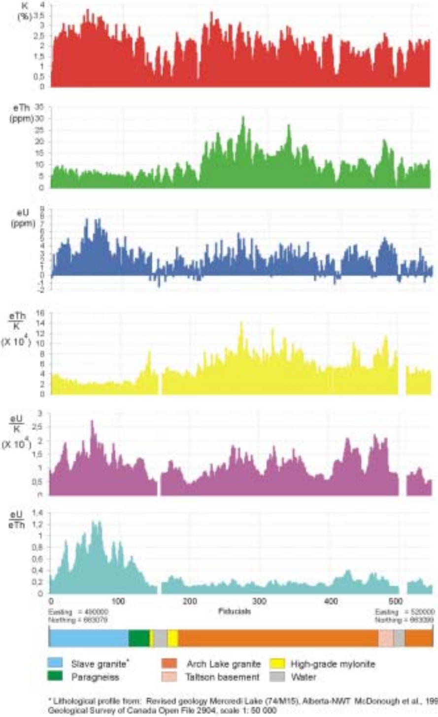
FIG. 7.2. Typical example of stacked airborne gamma ray spectrometer profiles showing K, eTh, eU, eTh/K, eU/K, eU/eTh and bedrock lithology. Airborne geophysical survey northeast Alberta, open file 2807 Geological Survey of Canada, Ottawa.
