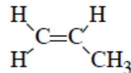
Propylene
