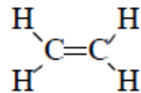
Ethylene
