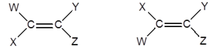
Geometric isomers
