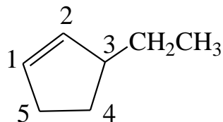
3-Ethylcyclopentene
