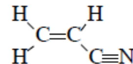
Acrylonitrile
