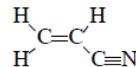
Acrylonitrile
