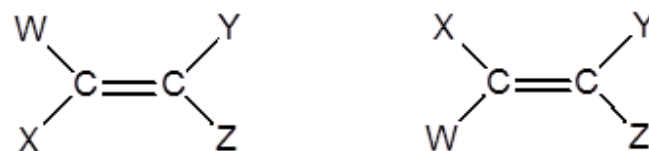
Geometric isomers
