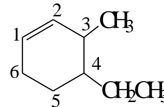
4-Ethyl-3-methylcyclohexene
