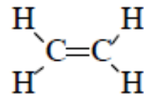
Ethylene
