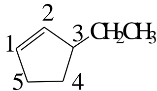
3-Ethylcyclopentene 5-Ethylcyclopentene
