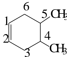
4,5-Dimethylcyclohexene
