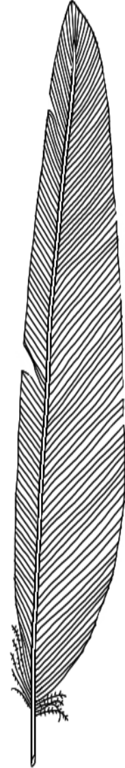
Contour feather
