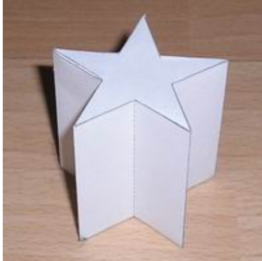
Pentagrammic Prism
