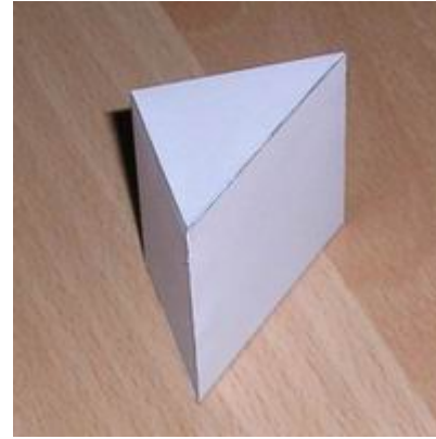
Triangular prism
