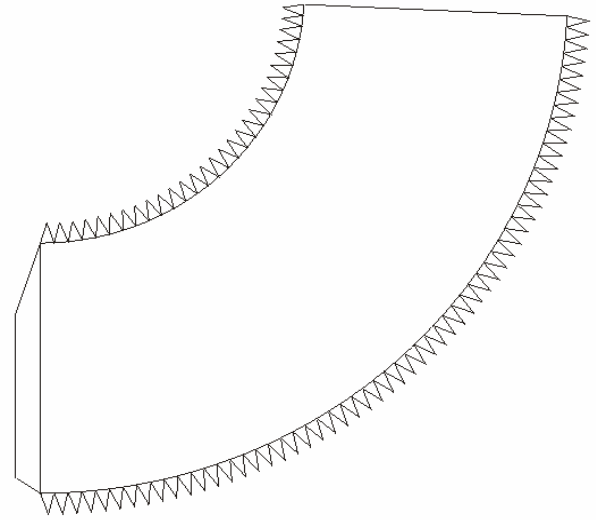
Tapered cylinder
