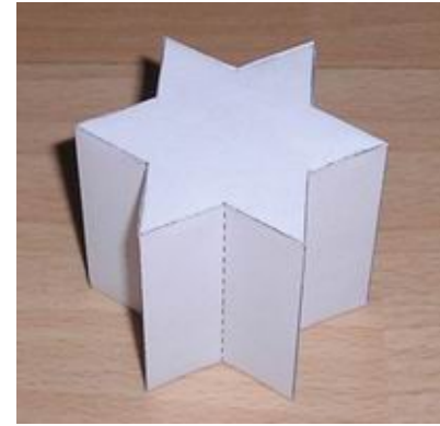
Hexagrammic Prism
