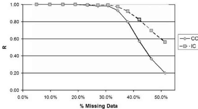
Fig. 5 Ability vs. proportion of missing data
