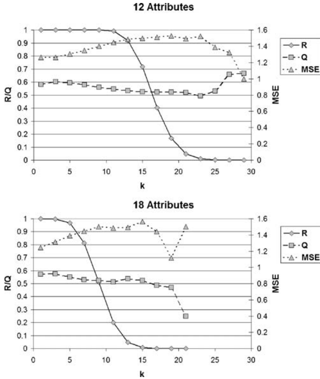
Fig. 4 9.9% missing data, 12 (top) and 18 (bottom) attributes, IC
