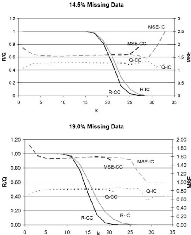
Fig. 3 Performance at 14.5 and 19% missing data, CC and IC
