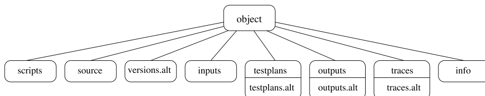
Figure 2. Object directory structure (top level).
