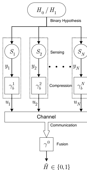
Figure 1: Parallel fusion network.
