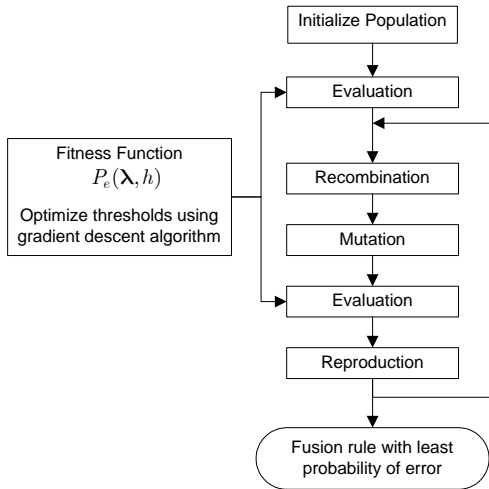
Figure 3: Sensor network optimization using the genetic algorithm.
