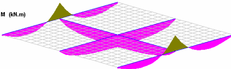
Figure 8 : Analysis and design of a stiffened plate – Internal forces in embedded beams
