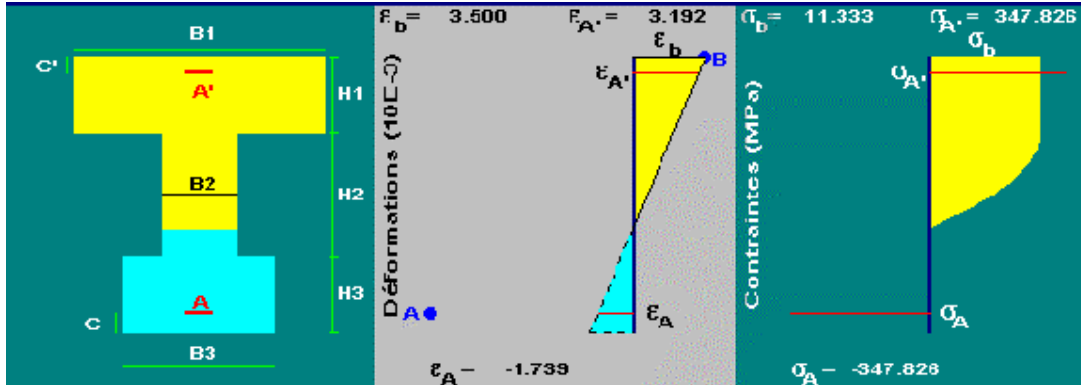
Figure 1 : RC design in ULS (Ultimate Limit State)
