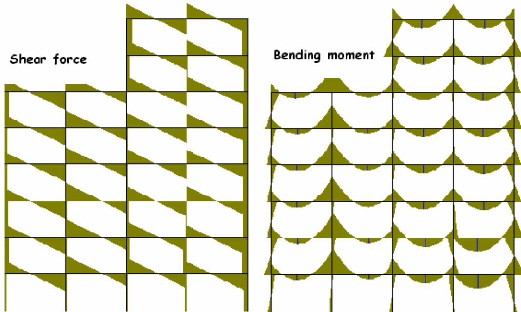
Figure 9 : Analysis and design of framed structures
