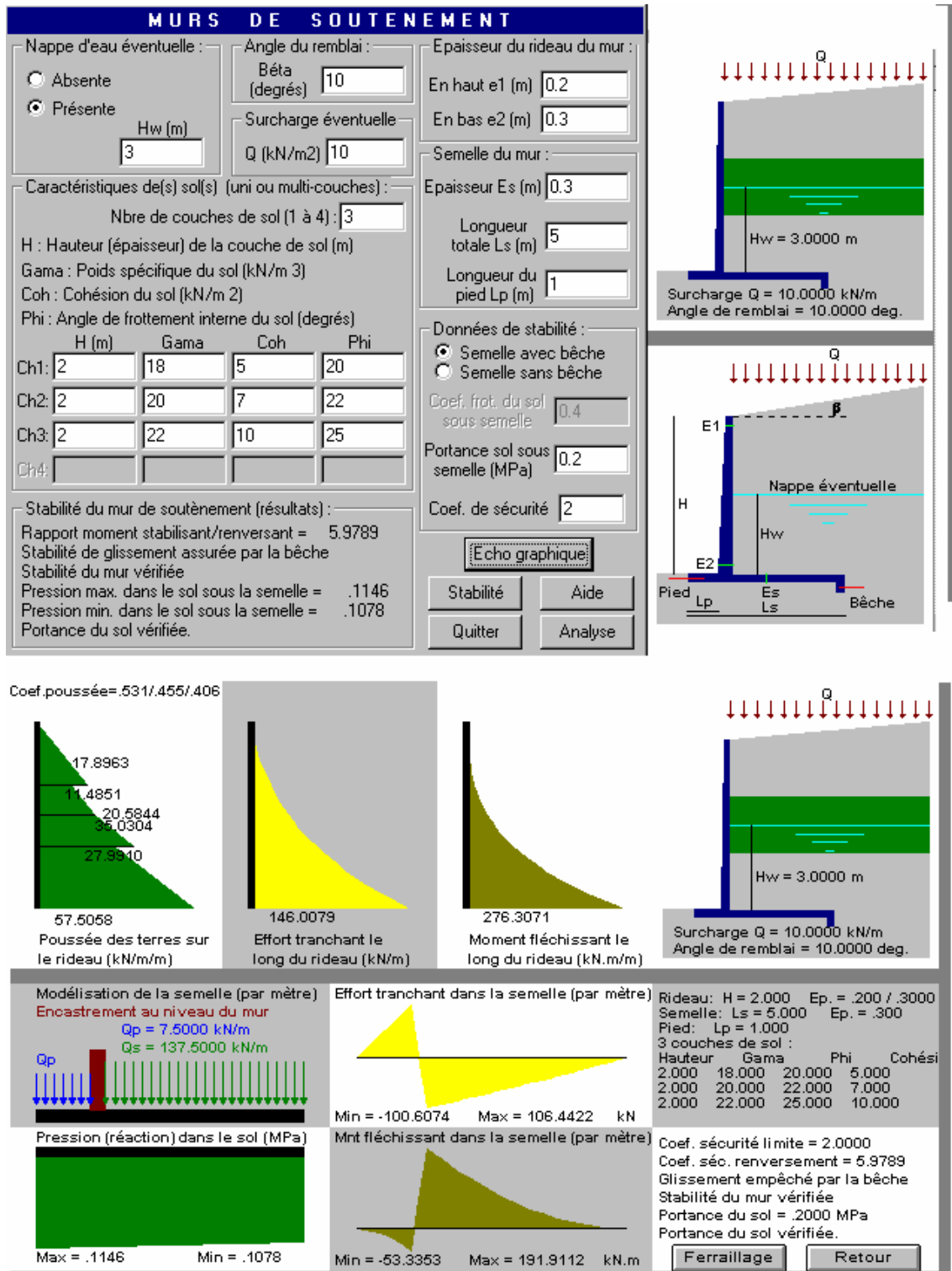
Figure 5: Analysis and design of retaining walls
