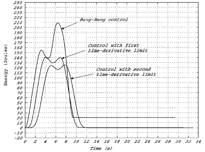
Fig. 9 Energy during and after a maneuver.
