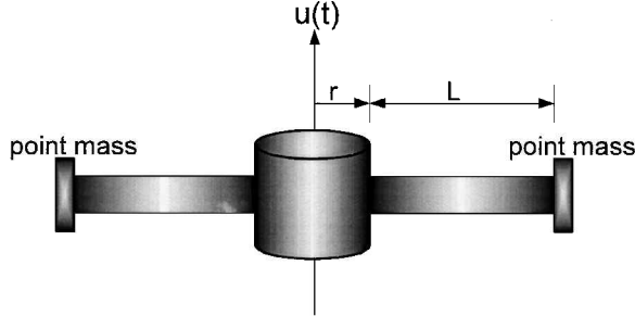
Fig. 5 Flexible structure.
