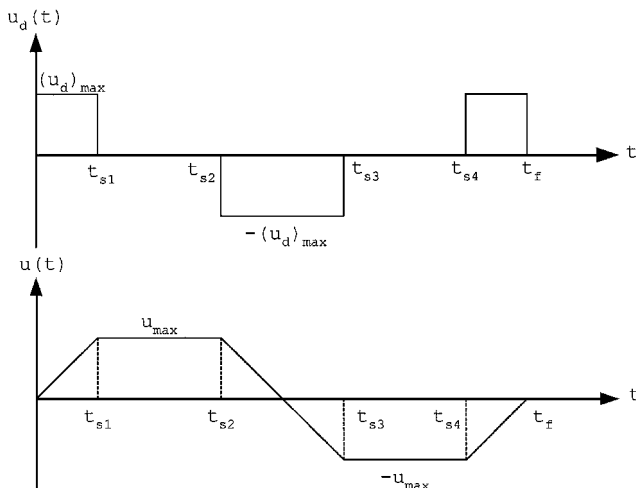
Fig. 1 Constrained time-optimal structure for u_d(t) and u(t) .
