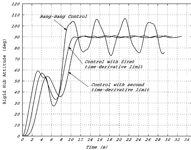
Fig. 8 Rigid-hub attitudes.
