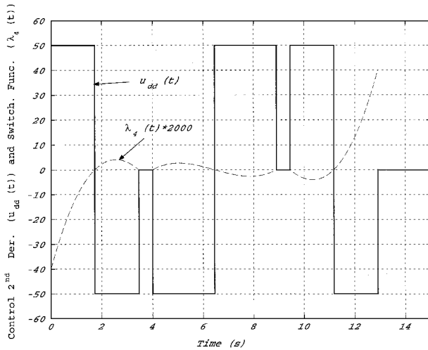
Fig. 12 Control with second time-derivative constraint and its switching function.
