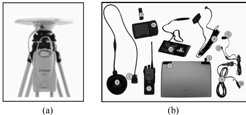
Fig.2. Survey equipments, (a) Trimble GPS Total Station 5700; (b) TETRA Propagation Survey Equipments
