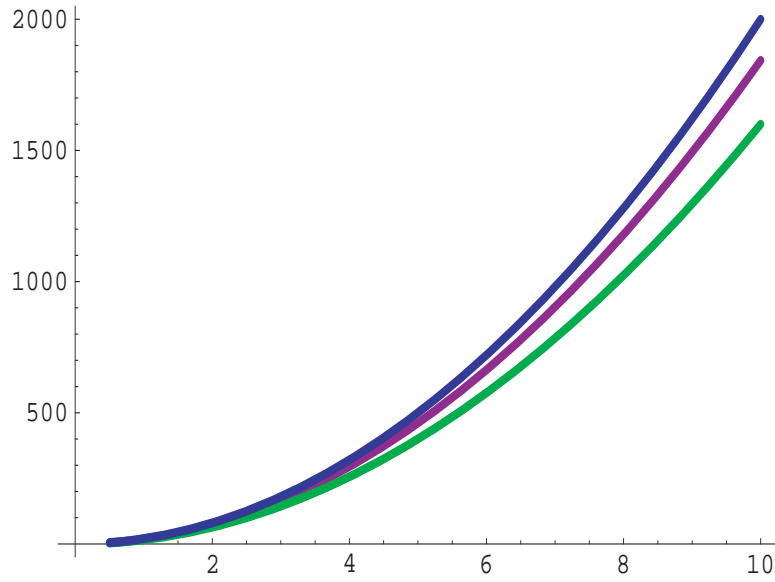
Figure 3.2: Information bounds, .5 \leq \alpha \leq 10 , \beta = .5 ; green = I^{-1}(P|\nu, \mathcal{P}_0) , purple = I^{-1}(P|\nu, \mathcal{P}) , blue = Var_{\theta}(X)
