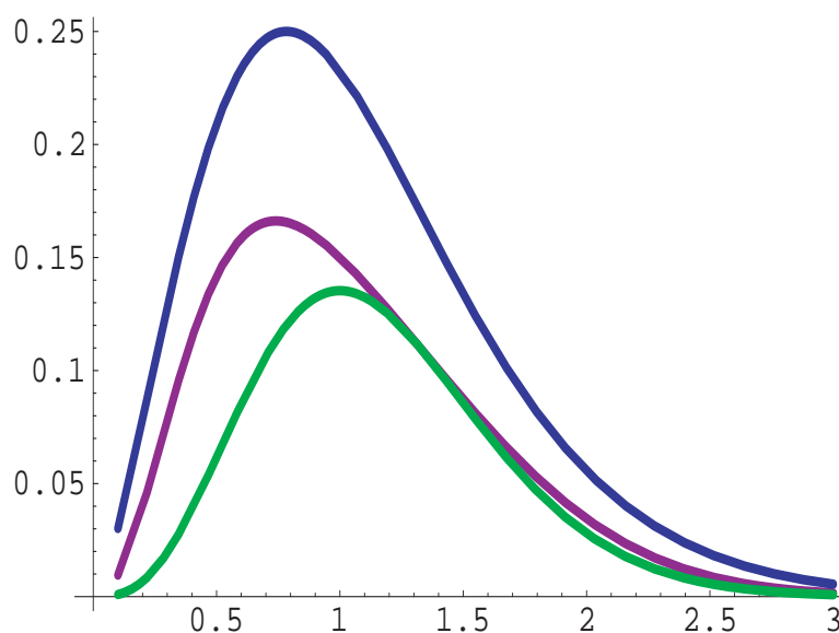
Figure 3.5: Information bounds for \nu(P_\theta) = P_\theta(X \geq x_0) , \alpha = 1 , \beta = 1.5 , .1 \leq x_0 \leq 3.0 ; green = I^{-1}(P|\nu, \mathcal{P}_0) , purple = I^{-1}(P|\nu, \mathcal{P}) , blue = nVar(\mathbb{F}_n(x_0)) = P_\theta(X \geq x_0)(1 - P_\theta(X \geq x_0))
