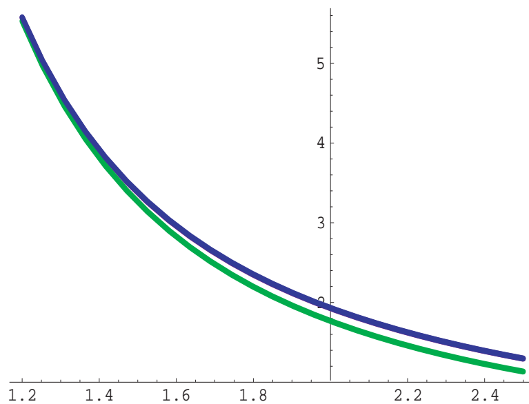
Figure 3.1: Information bounds, \alpha = 3 , 1.2 \leq \beta \leq 2.5 ; green = I^{-1}(P|\nu, \mathcal{P}_0) , purple = I^{-1}(P|\nu, \mathcal{P}) , blue = Var_{\theta}(X) ; (purple coincides with blue so not visible!)
