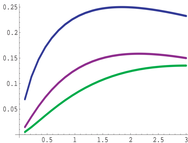
Figure 3.6: Information bounds for \nu(P_\theta) = P_\theta(X \geq x_0) , \alpha = 3 , \beta = .75 , .1 \leq x_0 \leq 3.0 ; green = I^{-1}(P|\nu, \mathcal{P}_0) , purple = I^{-1}(P|\nu, \mathcal{P}) , blue = nVar(\mathbb{F}_n(x_0)) = P_\theta(X \geq x_0)(1 - P_\theta(X \geq x_0))
