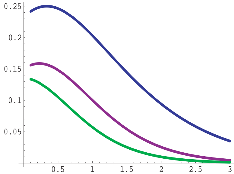
Figure 3.4: Information bounds for \nu(P_\theta) = P_\theta(X \geq x_0) , \alpha = 3 , x_0 = 1 , .1 \leq \beta \leq 3.0 ; green = I^{-1}(P|\nu, \mathcal{P}_0) , purple = I^{-1}(P|\nu, \mathcal{P}) , blue = nVar(\mathbb{F}_n(x_0)) = P_\theta(X \geq x_0)(1 - P_\theta(X \geq x_0))
