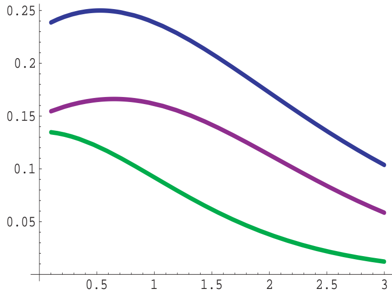
Figure 3.3: Information bounds for \nu(P_\theta) = P_\theta(X \geq x_0) , \alpha = 1 , x_0 = .5 , .1 \leq \beta \leq 3 : green = I^{-1}(P|\nu, \mathcal{P}_0) , purple = I^{-1}(P|\nu, \mathcal{P}) , blue = nVar(\mathbb{F}_n(x_0)) = P_\theta(X \geq x_0)(1 - P_\theta(X \geq x_0))
