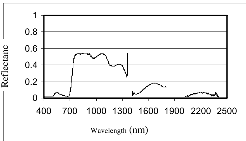
Figure 4. Spectral reflectance of alfalfa under 50 cm water table
