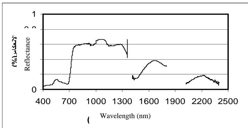
Figure 3. Spectral reflectance of alfalfa under 100 cm water table
