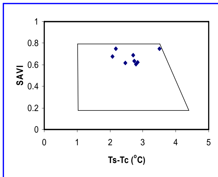
Figure 6. Temperature difference – SAVI trapezoid of alfalfa grown under varying watertable depths
